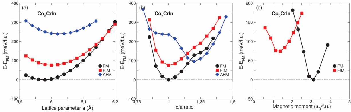
Fig. 2. Dependence of total energy per formula unit on (a) lattice parameter, (b) tetragonality degree c/a and (c) fixed total magnetic moment of \text{Co}_2\text{CrIn} alloy with FM, AFM, and FIM configurations. The energy difference was calculated with respect to the stable configuration (FM)
