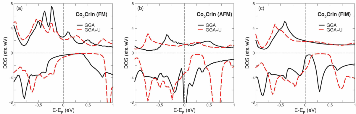
Fig. 4. Total DOS curves for spin up and spin down bands of Co 2 CrIn alloy near the Fermi level in (a) FM, (b) AFM, and (c) FIM spin configurations. Solid (dashed) lines denote results for GGA (GGA+ U ) approach
